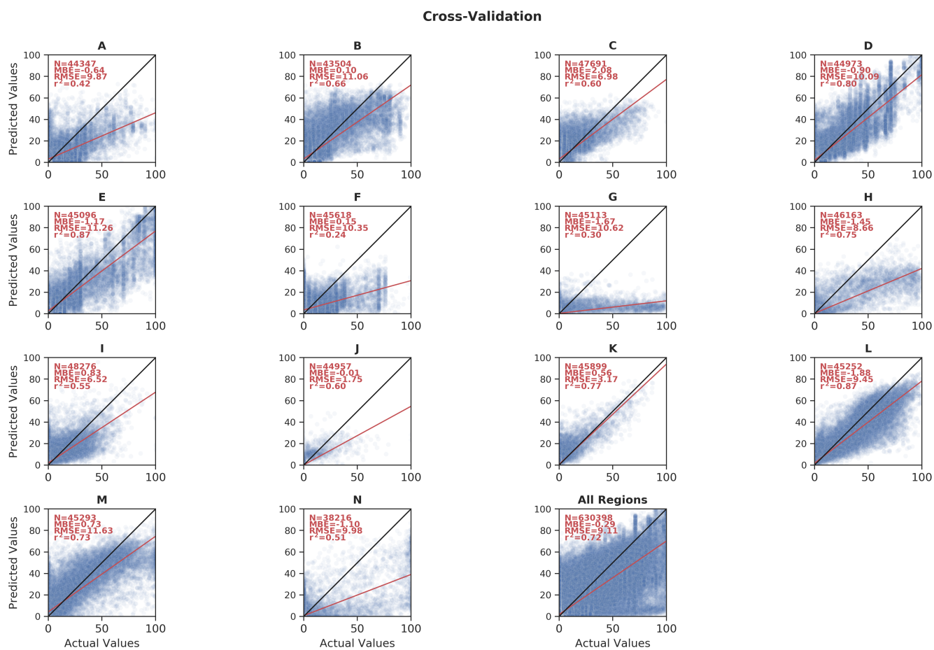
Figure A4. Scatter plots of the CV trials for Peat-ML (Peat-ML CV) predicted peatland extent and extent from the peatland training datasets over the 14 BLOO CV blocks.
