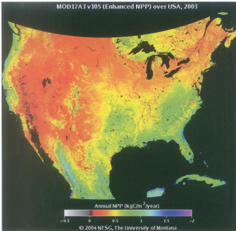
Figure 2. Net primary production (NPP) for the US for 2003. Some parameters for an aggregate index of ecosystem services, such as NPP, are relatively easy to assess for the entire US, while services are more regionally or locally specific.
